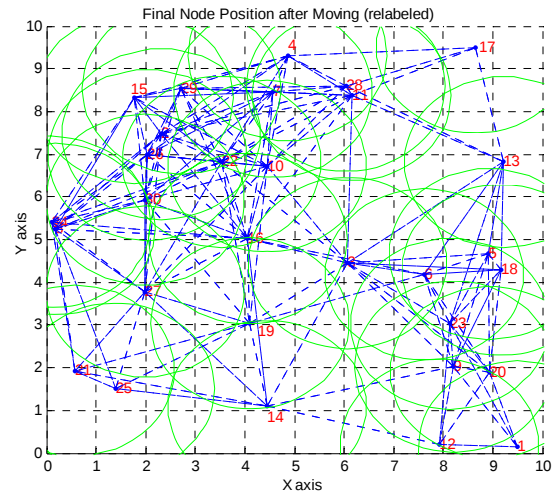
Fig. 6. Final node positions after executing proposed movement-assisted deployment algorithm
