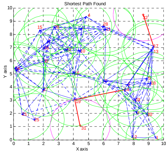
Fig. 5. Find shortest path by Dijkstra's algorithm from redundant node to virtual node point
