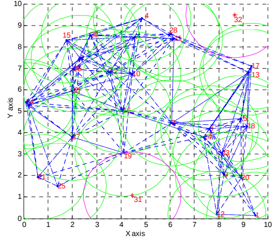
Fig. 4. Determine virtual node point in uncovered area and redundant nodes
