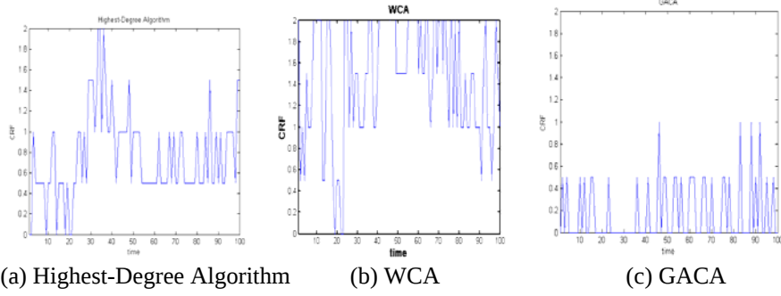
Fig.3. CRF under various clustering algorithms
