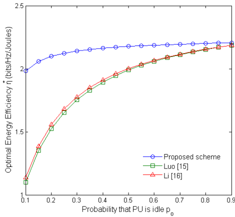
Fig. 9. Comparison of optimal energy efficiency.
