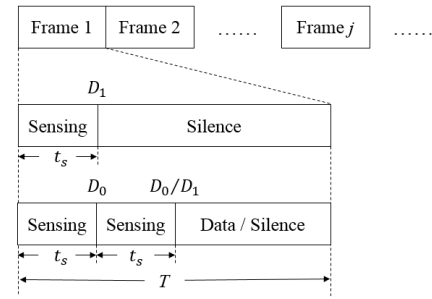
Fig. 2. Frame structure of spectrum sensing.
