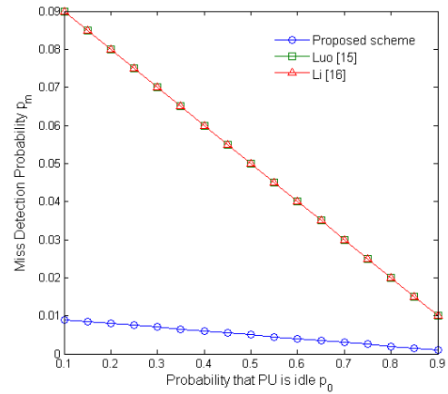
Fig. 11. Comparison of miss detection probability.
