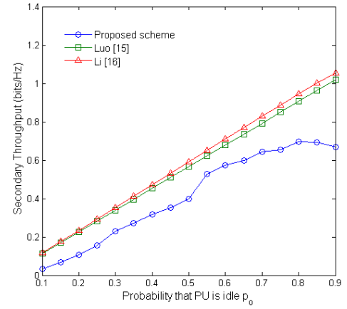
Fig. 10. Comparison of secondary throughput.
