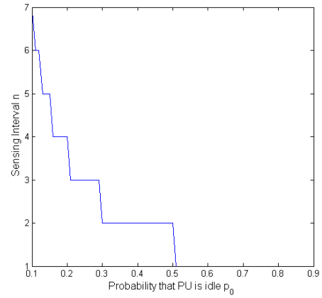
Fig. 7. The sensing interval as a function of p_0 .
