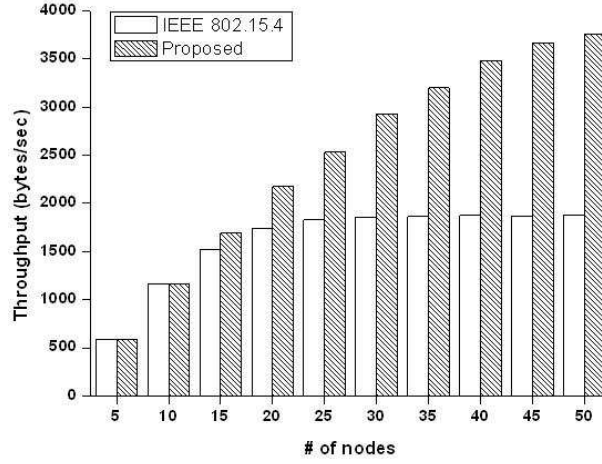
Figure 5.3: Throughput comparison (medical devices).
