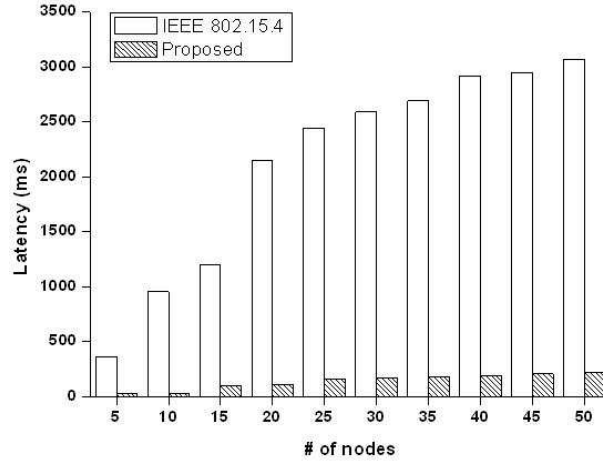
Figure 5.5: Latency comparison (CE device).
